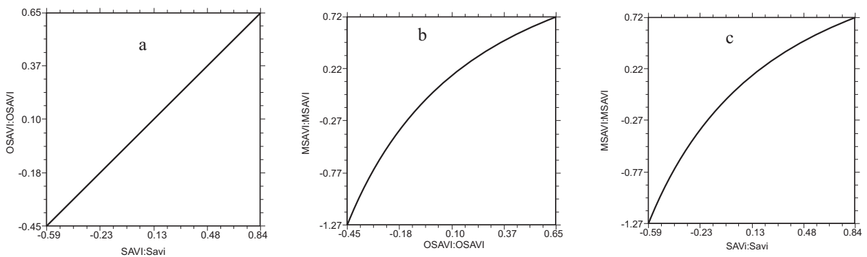
Fig. 5. Vegetation indices scatter plots: a – OSAVI-SAVI, b – MSAVI2-OSAVI, c – MSAVI2-SAVI.
