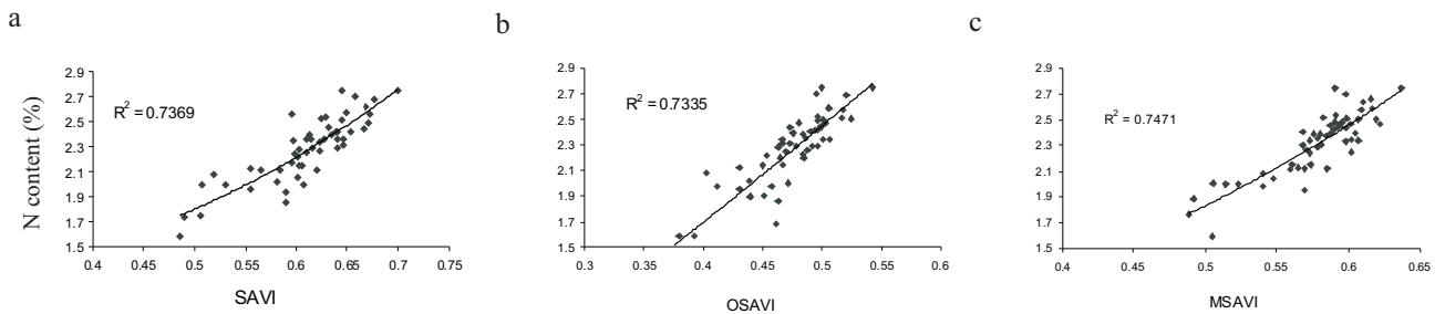
Fig. 4. Relationship between corn nitrogen content and: a – SAVI, b – OSAVI, c – MSAVI2.
