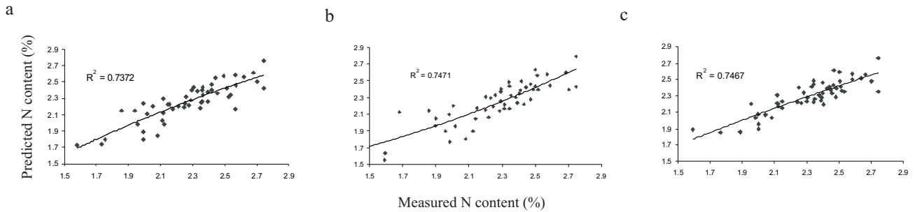
Fig. 6. Relationship between measured and predicted corn nitrogen content with : a – SAVI, b – OSAVI, c – MSAVI2.
