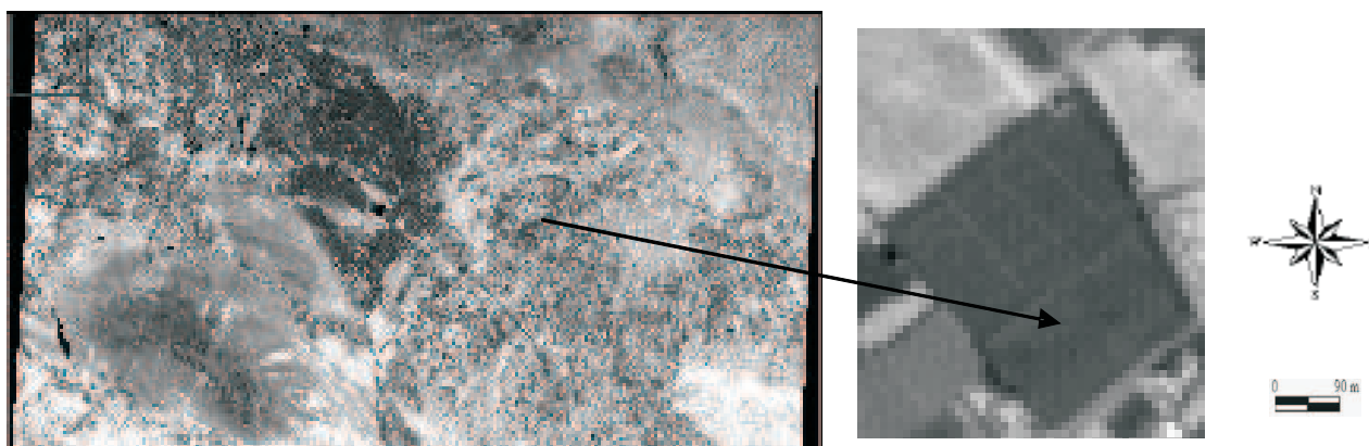
Fig. 1. FCC (3-2-1 composition) imagery of ASTER sensor of the studied area.
