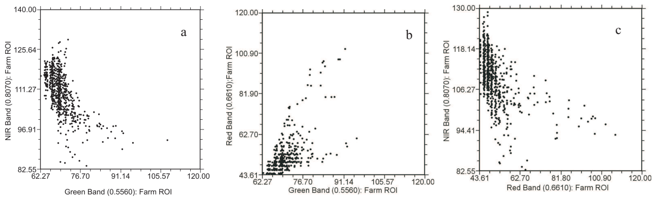
Fig. 3. NIR, red and green scatter plots.
