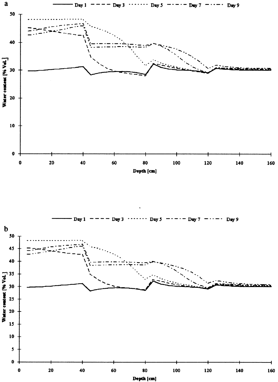
Fig. 3. Numerical test of the crack submodel without cracks (a), and with crack influence on the bypass flow (b) for third variant of initial water content.
